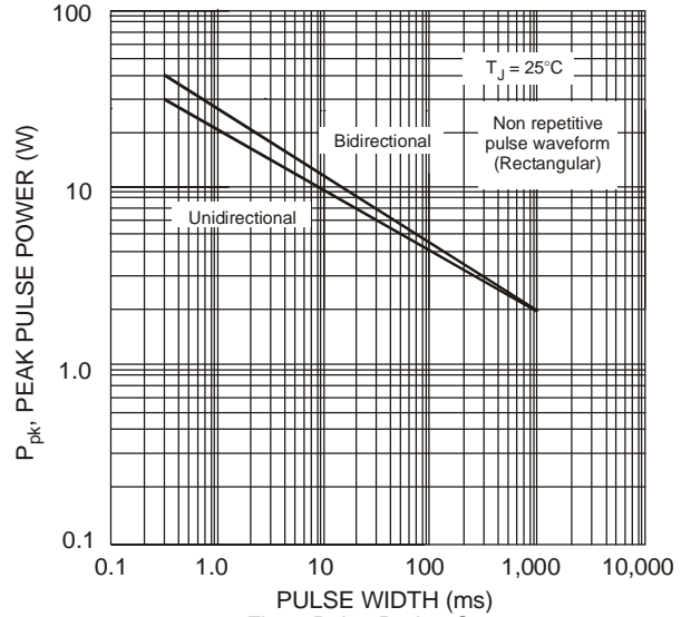
Fig. 6 Pulse Rating Curve, P_{pk} (W) vs. Pulse Width (ms) Power is defined as P_{pk} = V_C \times I_{pp}
